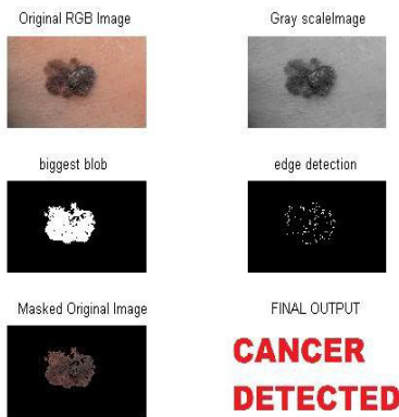
Fig.6 Cancer detected
