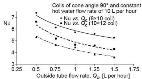
Figure 9. Variation of Nusselt number with outside tube fluid flow rate, Q_c , with coils of different tube diameter, d_i
