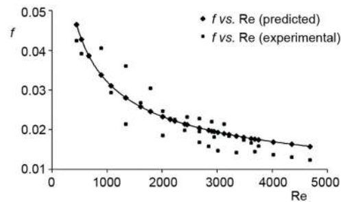
Figure 12. Comparison of friction factor, f , vs. Reynolds number for predicted and experimental values
