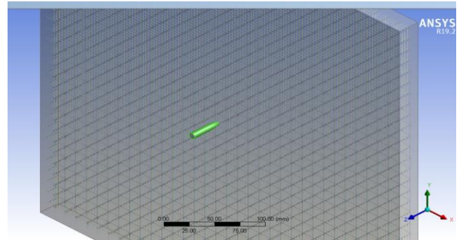
Fig. 1: Modelling High Impact Analysis Setup
