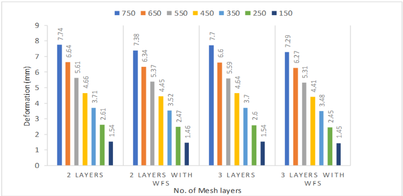
Graph 1: Deformation in (mm) For 15mm thick Ferrocement Panel.
