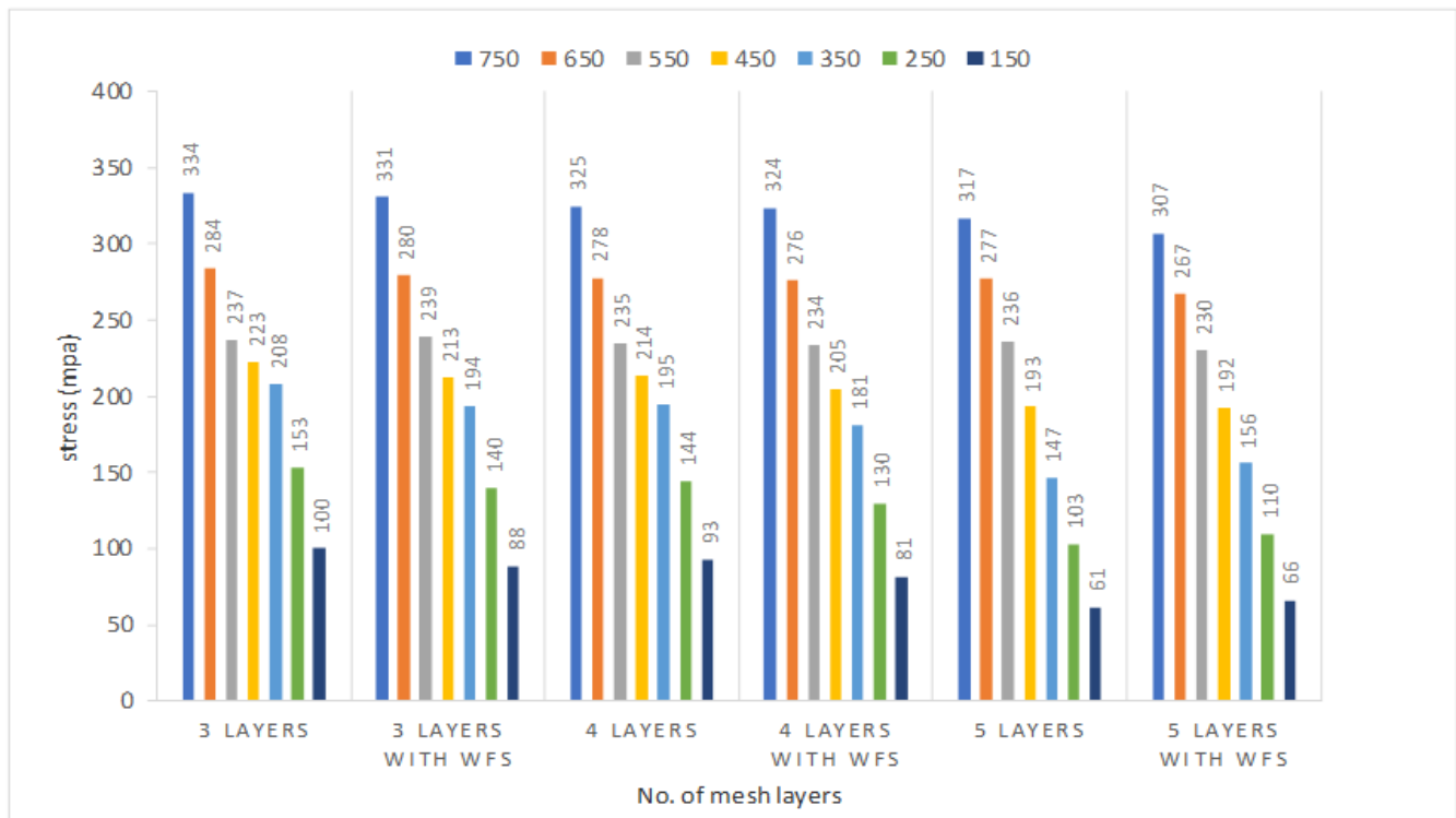
Graph 6: Equivalent Stress in (MPa) for 25mm thick Ferrocement Panel
