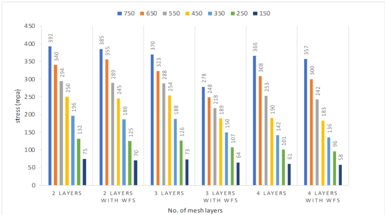
Graph 5: Equivalent Stress in (MPa) for 20mm thick Ferrocement Panel.
