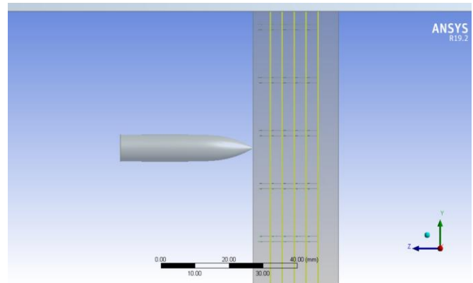
Fig. 2: Cross section showing wire-mesh layers
