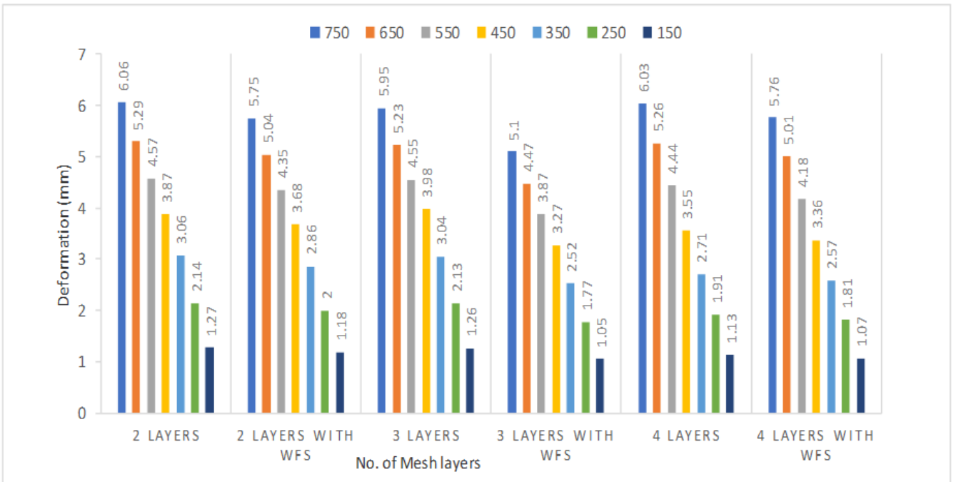
Graph 2: Deformation in (mm) For 20mm thick Ferrocement Panel
