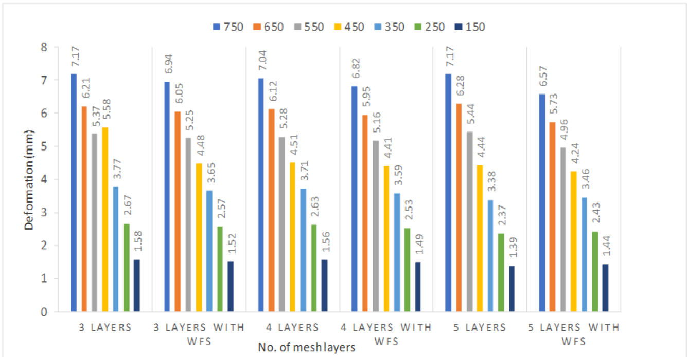
Graph 3: Deformation in (mm) For 25mm thick Ferrocement Panel
