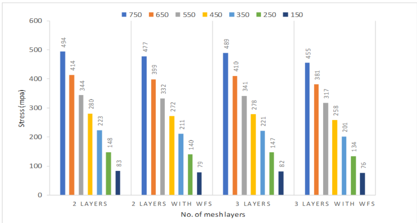
Graph 4: Equivalent Stress in (MPa) For 15mm thick Ferrocement Panel
