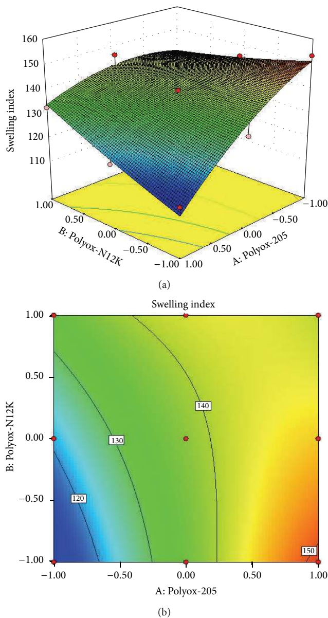
FIGURE 7: (a) Response surface plot showing the influence on swelling index and (b) contour plot.
