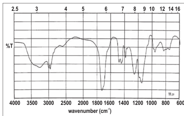
Figure 2: FTIR spectra of eudragit S-100
