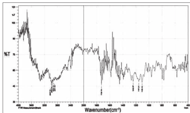
Q1 Figure 3: FTIR spectra of physical mixture of eudragit S-100 and propranolol HCl
